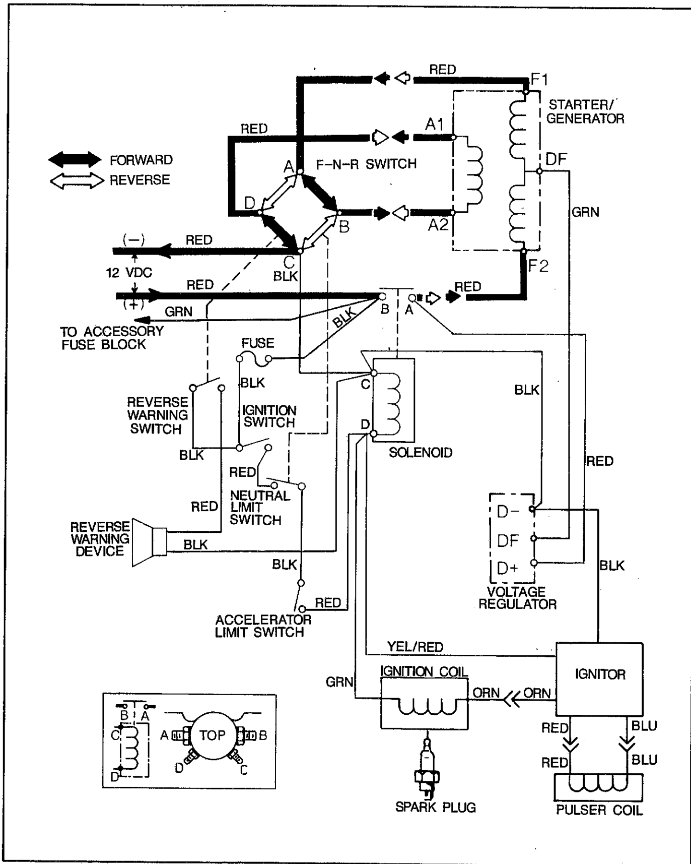
FIG. L-2 ELECTRICAL SYSTEM WIRING DIAGRAM – 1989/ EARLY 1990
